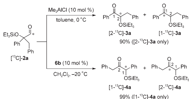
Scheme 4. 1,2-Rearrangement of the 13 C-labeled substrate [ 13 C]- 2a .
