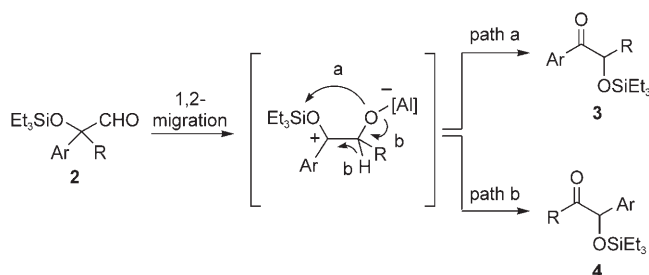
Scheme 3. The two possible reaction pathways.
