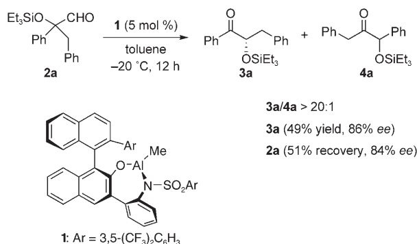
Scheme 1. 1,2-Rearrangement of the differently \alpha,\alpha -disubstituted \alpha -siloxy aldehyde 2a .
