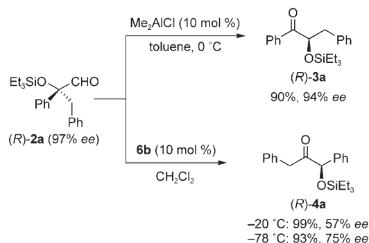
Scheme 2. 1,2-Rearrangement of optically active \alpha -siloxy aldehyde ( R )- 2a .
